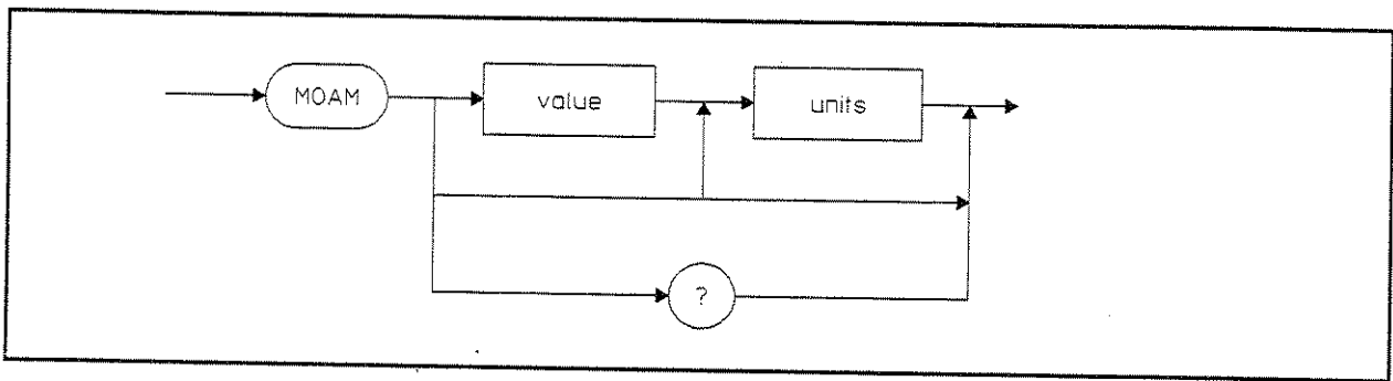
Figure 2-28. MOAM Syntax Diagram
